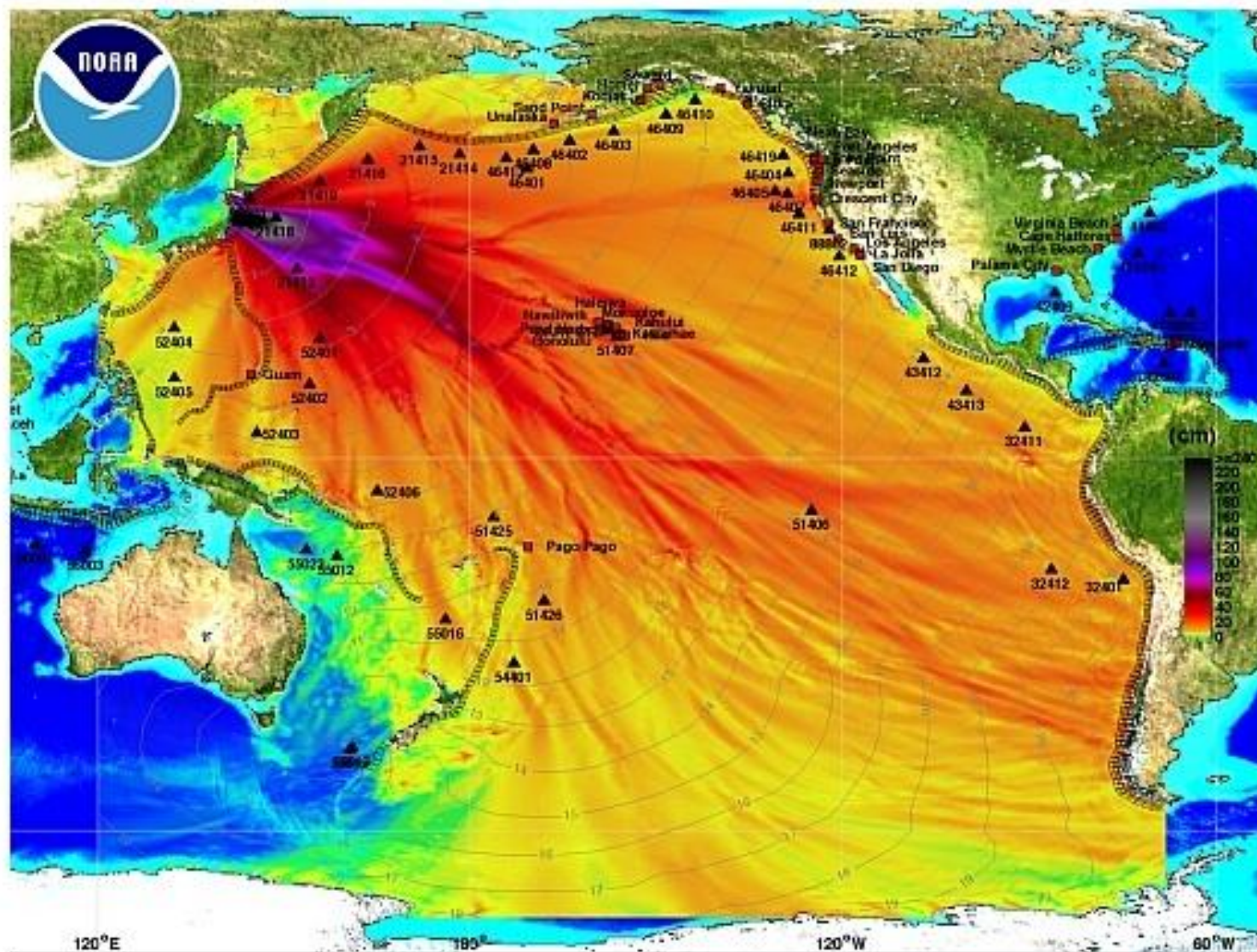
Energy propagation pattern of the 11 Mar 2011 tsunami. source: NOAA
